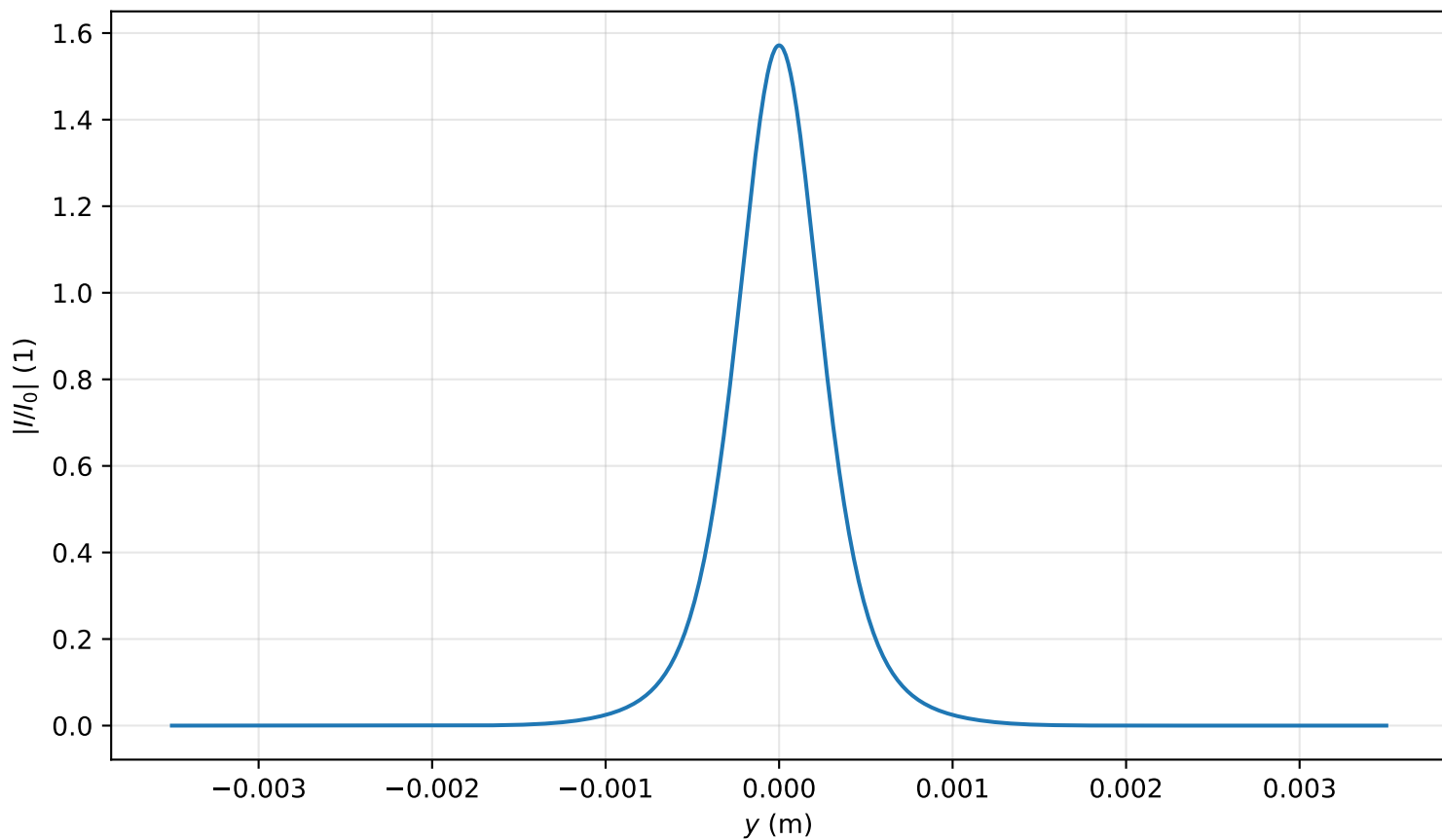
Intensity profile I(x = 0, y, z = 1.513)/I_0 , P_{in}=0.9P_{cr} , artificial time
